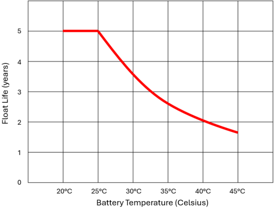
Float Service Life @ 25°C
